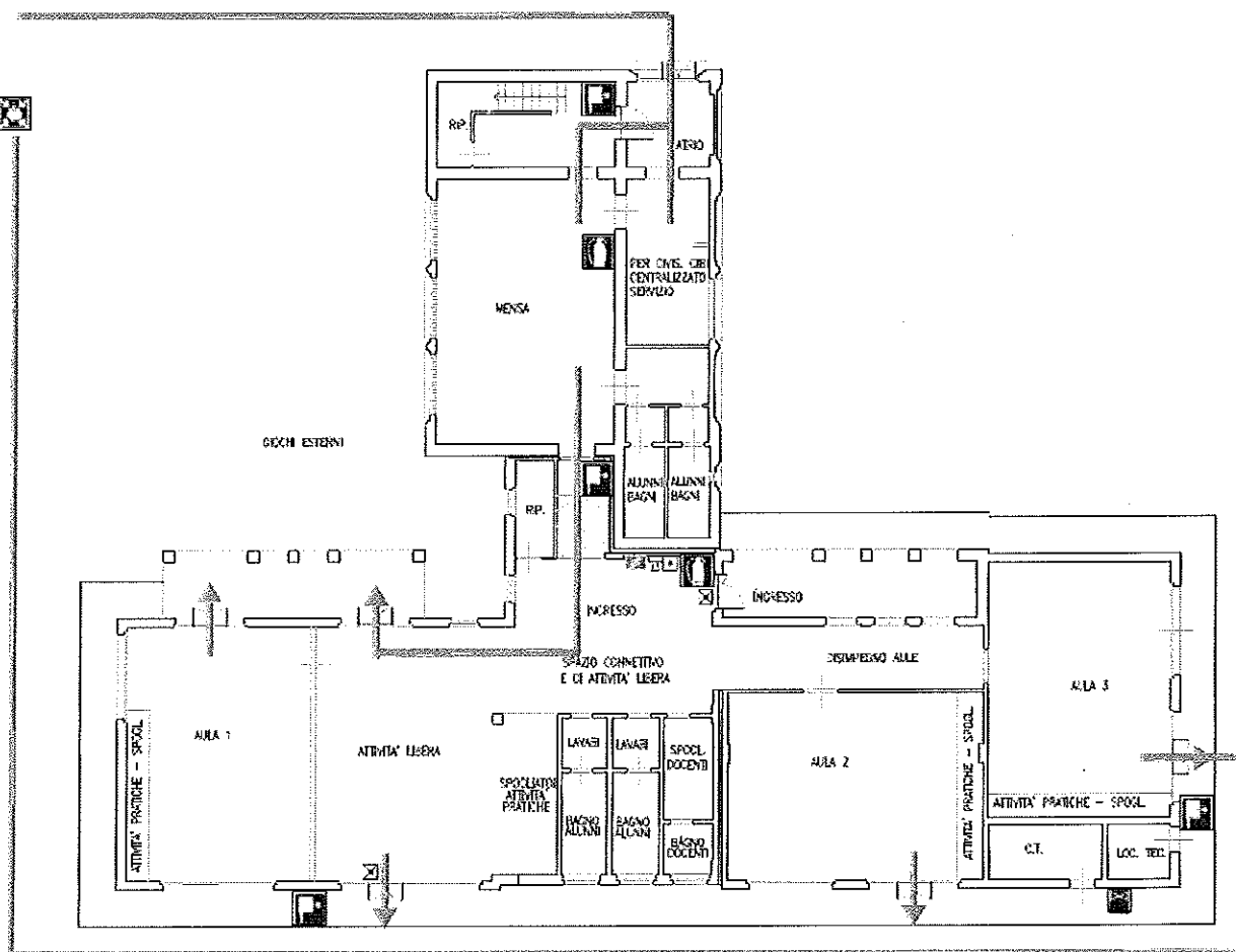
Piano Terra
